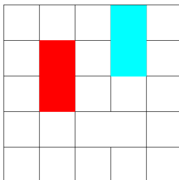
Figure 357: How the Randomized Kruskal's Algorithm Works (3/6)
